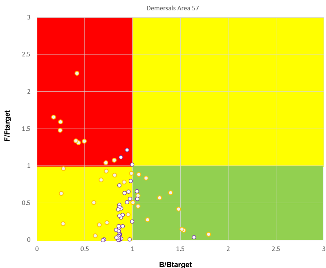
Figure 10.2.1. Kobe plot for F/F_{\text{target}} and B/B_{\text{target}} for Tier 1 (orange circles) and Tier 2 (purple circles) assessments of trawl-caught species collated at the workshop in January 2023.
