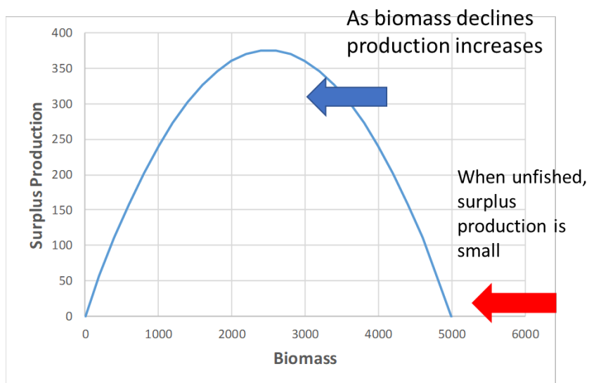
Figure 4.5. Basis for the biomass dynamic model for assessing fish stocks
