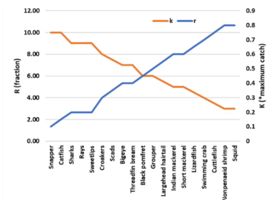
Figure A7.3. r and K priors scaled to the stock's PSA from a high K /low r ( 10 * \text{maximum catch}/0.1 ) to low K /high r ( 3 * \text{maximum catch}/0.8 )
