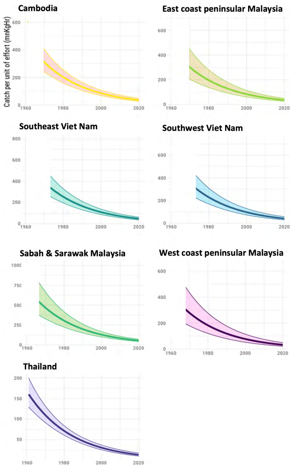
Figure 6.1. Standardized CPUE for seven areas in Southeast Asia based on research surveys conducted from 1960 to 2020
