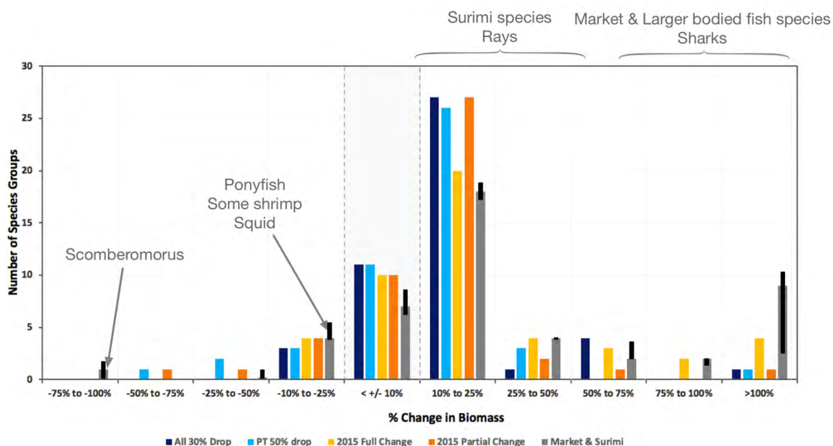
Figure 5.7. Proportional changes in production biomass under different scenarios of fishing effort in Thai waters of the Gulf of Thailand
