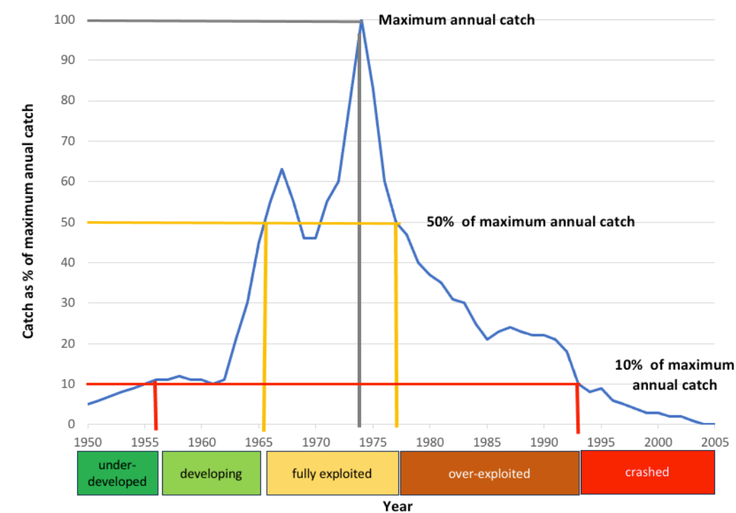
Figure 4.8. Classification of status of stocks based on catch trends from fishery data
