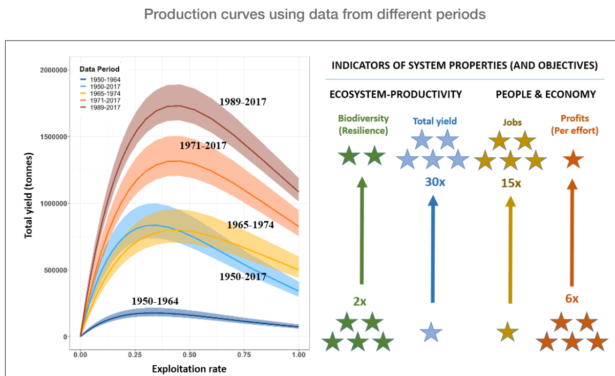
Figure 5.4. Aggregate production curves fit to various catch time series for the Gulf of Thailand. The different curves come from fitting to different time periods (and ecosystem states). The associated characteristics of those systems are summarized using indicators for biodiversity (and ecosystem resilience), total yield, jobs (employment) and profits per unit effort. The number of stars on the right of the plot shows the relative size of the various indicators for system properties that people often care about or hold as objectives
