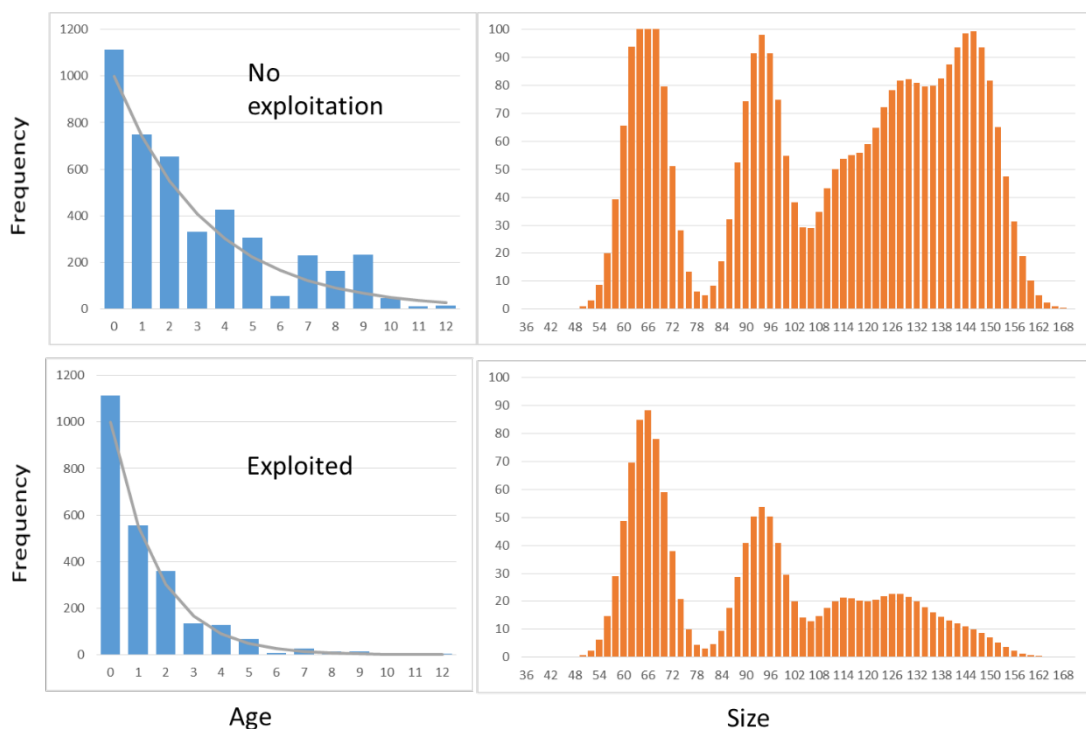
Figure 4.10. Examples of changes in the age and size distribution of an exploited and unexploited stock
