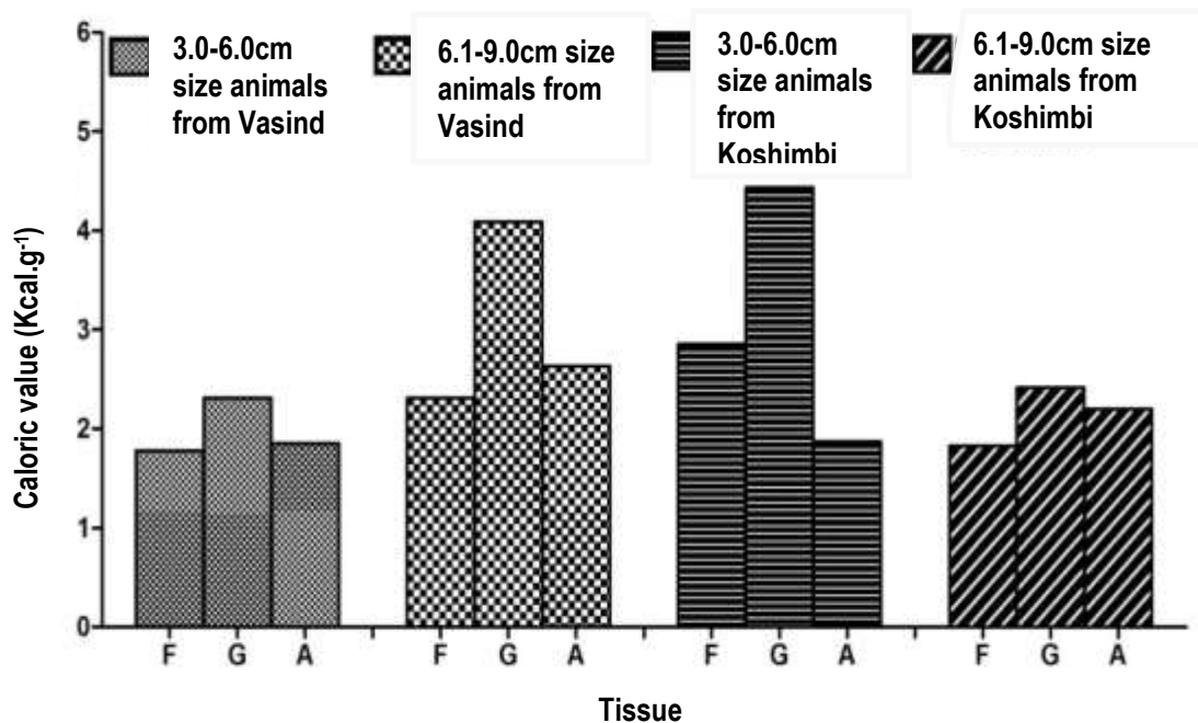
Fig. 5. Average caloric content value (Kcal.g -1 ) in foot (F), gill (G) and adductor muscle (A) tissues of 3.0 – 6.0 cm and 6.1 – 9.0 cm sizes of L. corrianus from Vasind and Koshimbi sampling sites
